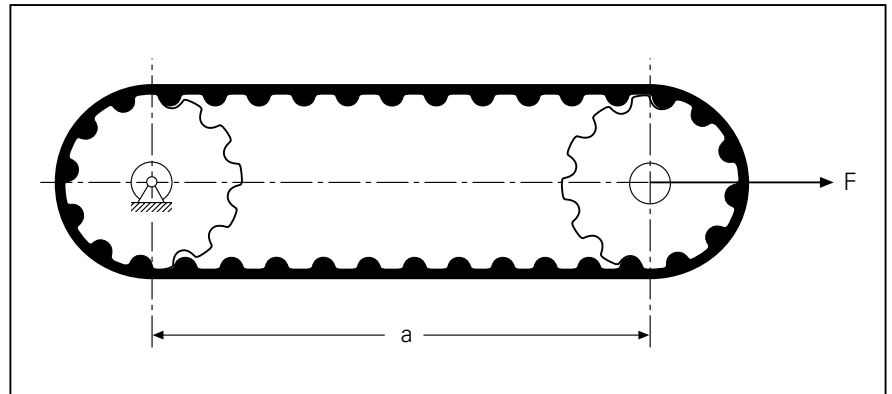
Measuring configuration
