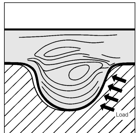
Stress distribution in the CONTI SYNCHROBELT® HTD tooth
