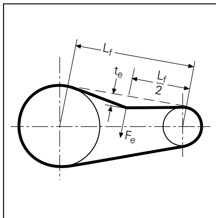
Belt deflection t_e Fig. 5
