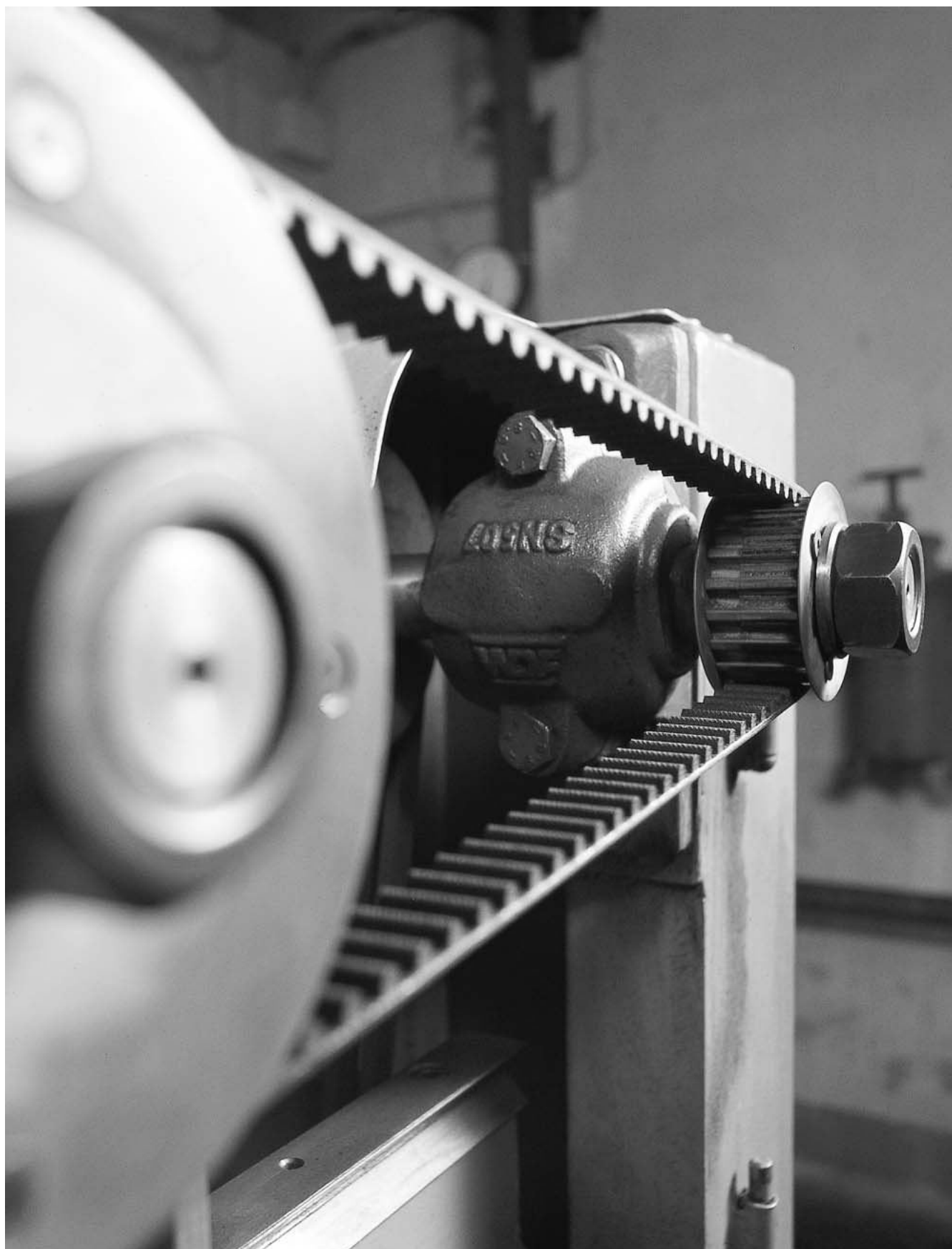
CONTI SYNCHROBELT® HTD synchronous drive belt being fatigue and performance-tested
