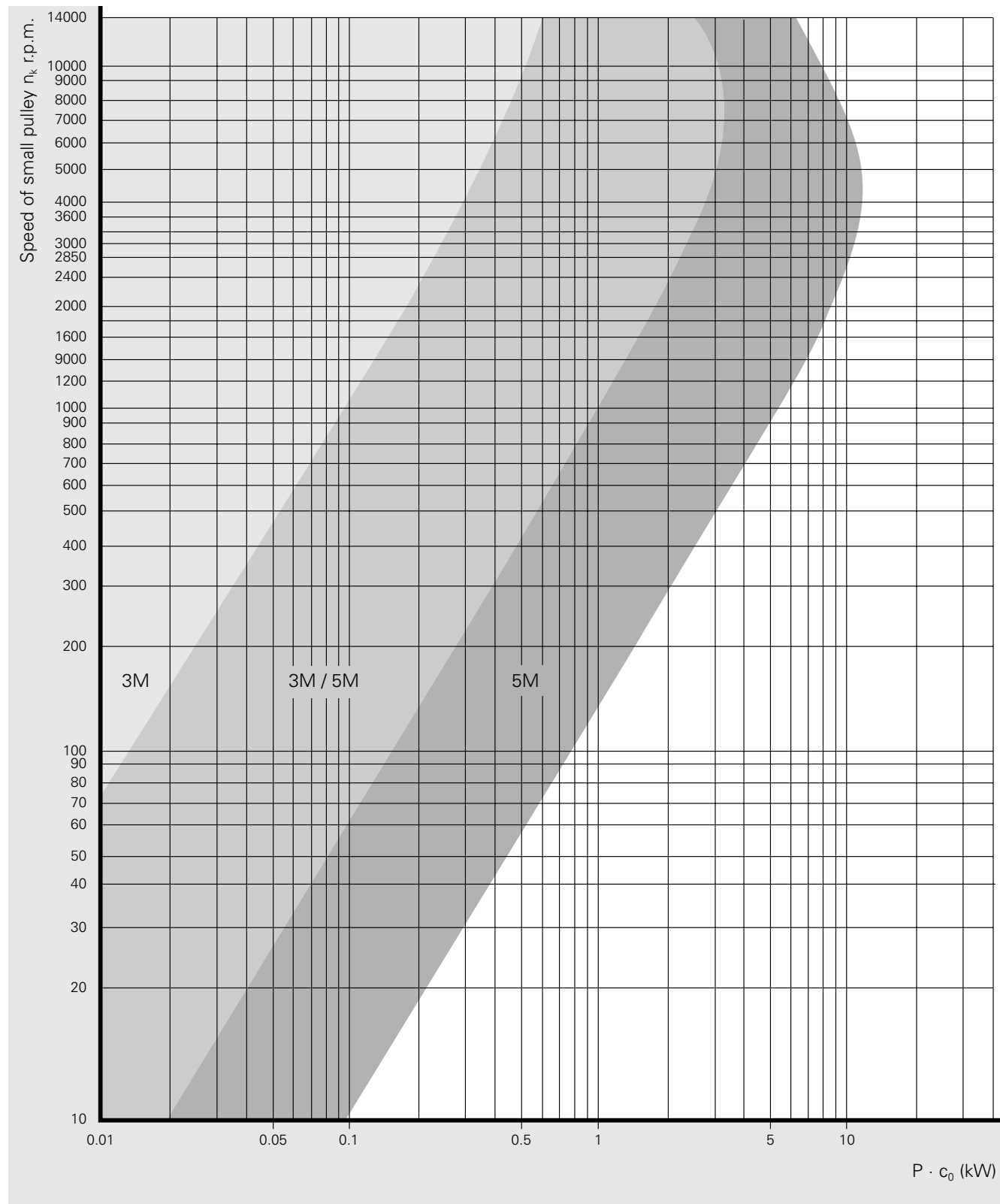
CONTI SYNCHROBELT® HTD Synchronous Drive Belt 3M, 5M
