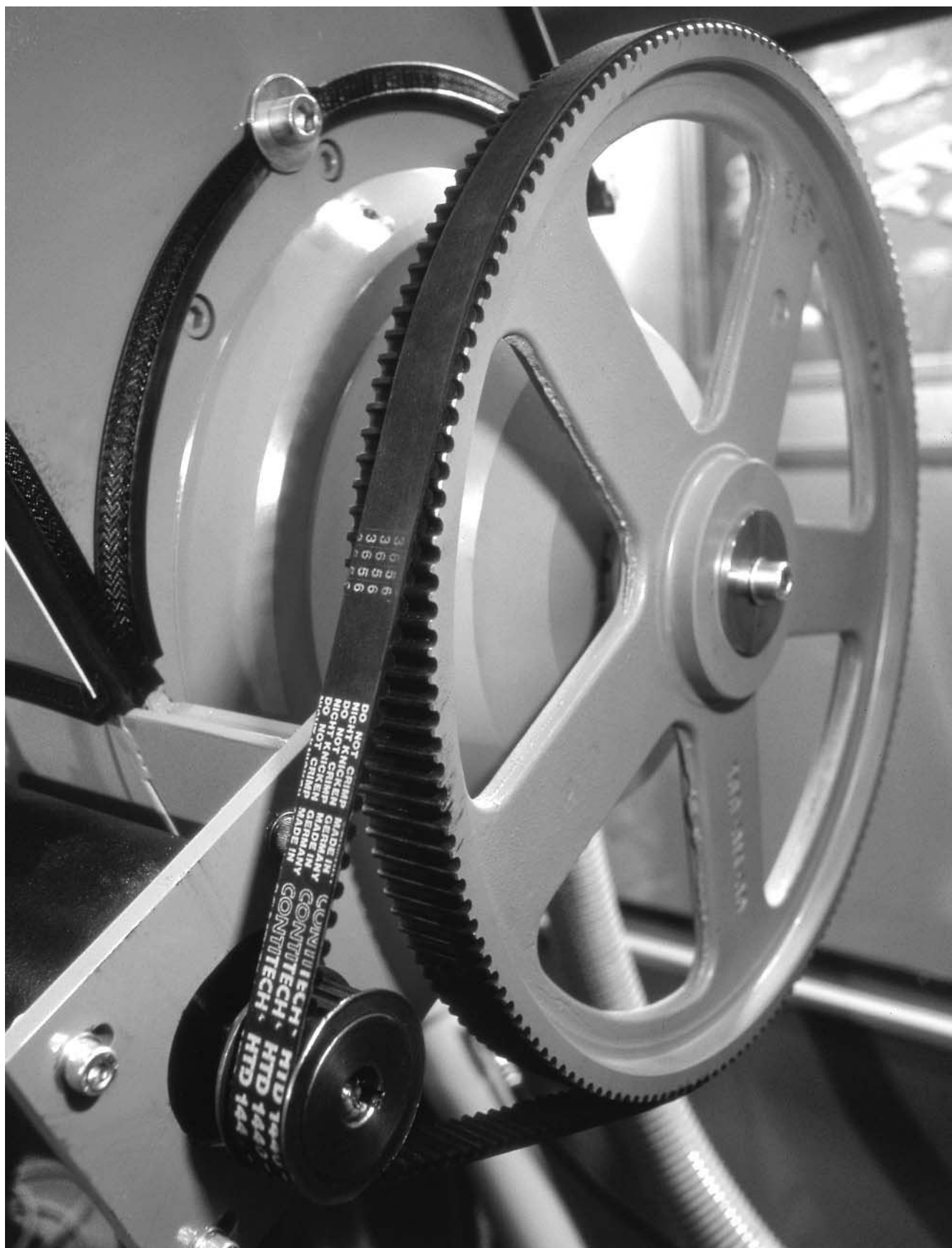
CONTI SYNCHROBELT® HTD synchronous drive belt on a grinding machine.
