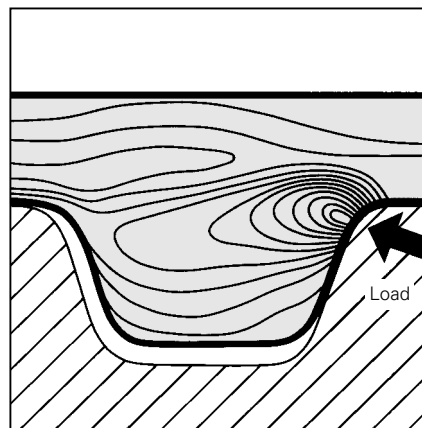
Stress distribution in the trapezoidal tooth
