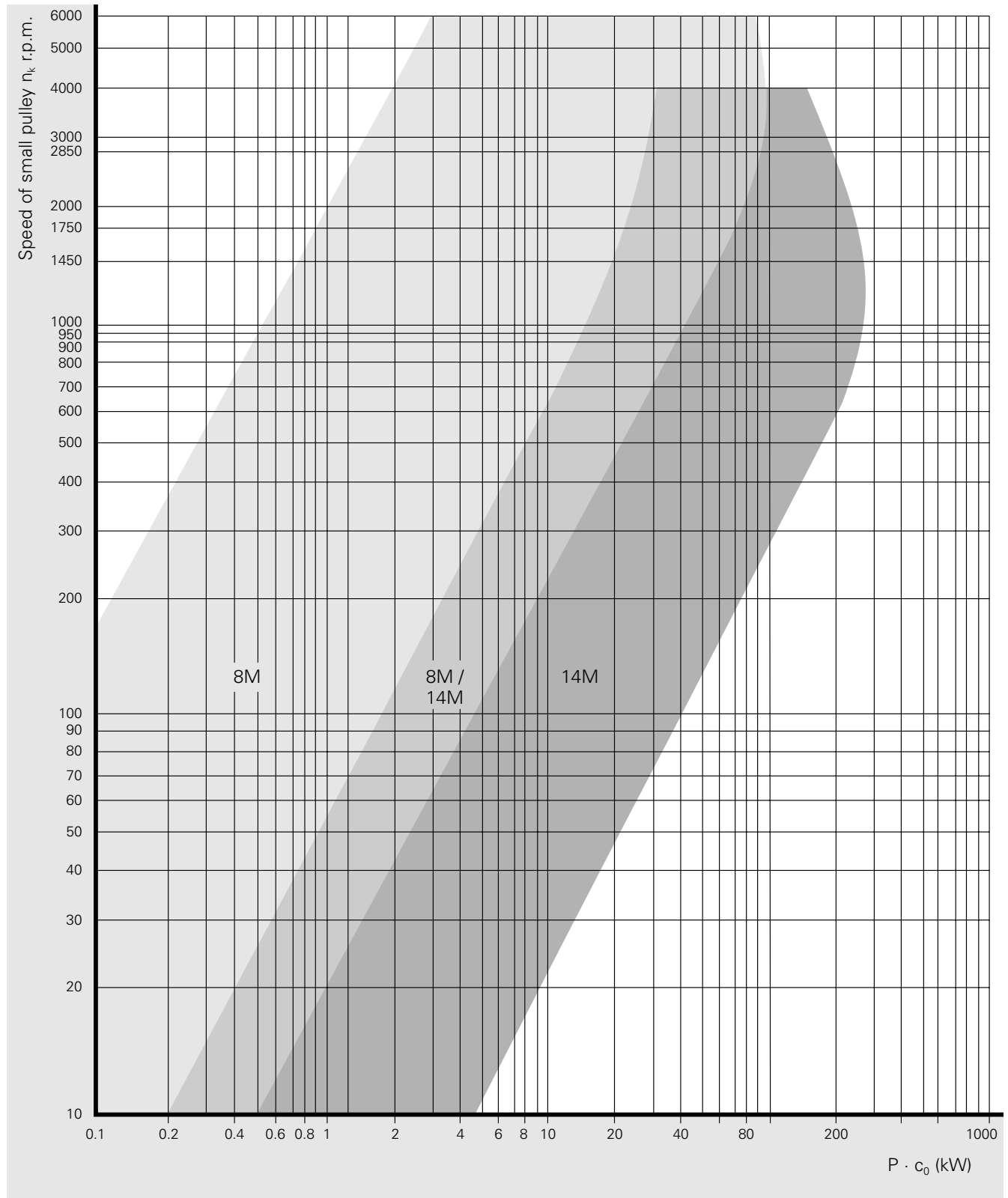
CONTI SYNCHROBELT® HTD Synchronous Drive Belt 8M, 14M
