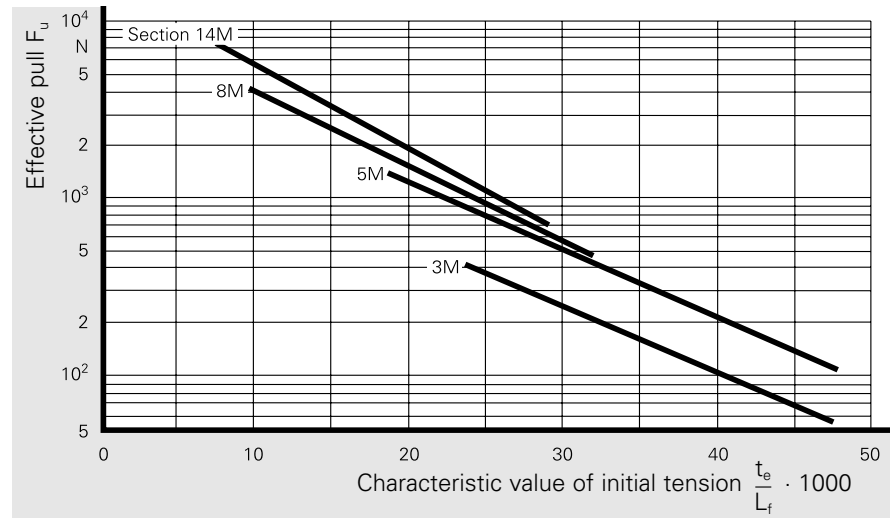
Characteristic lines of initial tension
