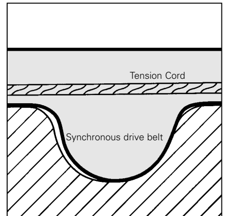
CONTI SYNCHROBELT® HTD tooth profile
